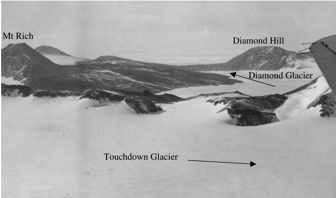
Arrows denote direction of glacier flow.
