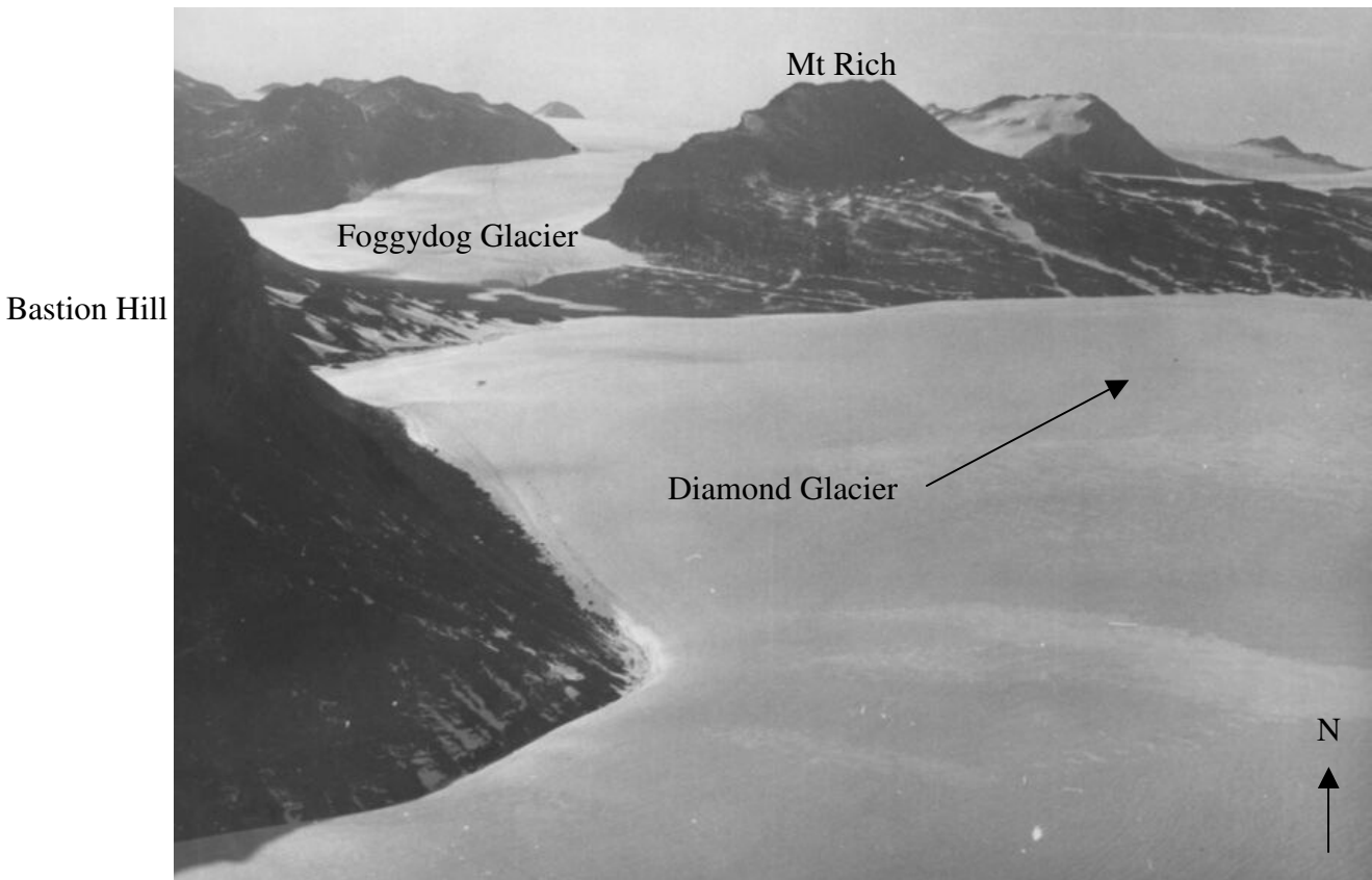
Arrows denote direction of glacier flow.
